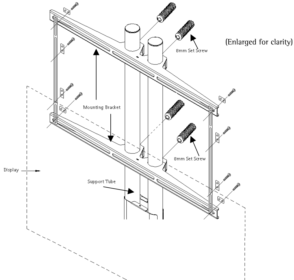
Figure 6. Mounting Bracket Installation
